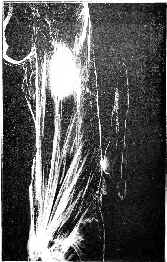
FIRE FOUNTAINS IN HALEMAUIMAU, KILAUEA
